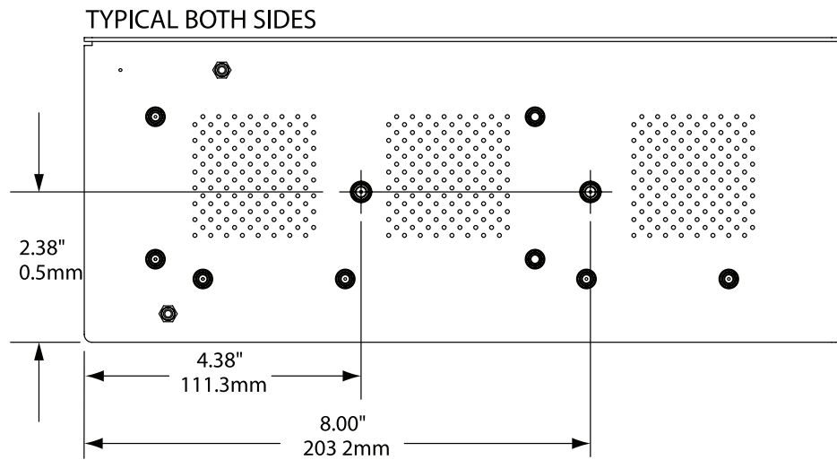
FIGURE 6. ASM-1 Smart Manifold Rack Slide Rail Mount Hole Dimensions.
