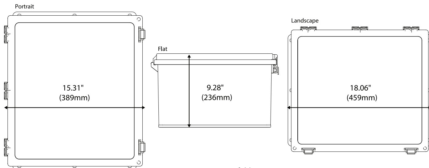
FIGURE A3. Smart Manifold AC NEMA Mounting Positions.
