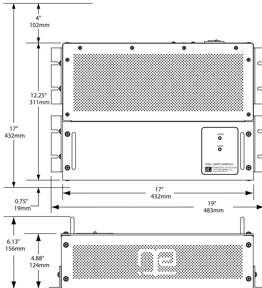
FIGURE 12. ASM-1 Smart Manifold Wall Mount Overall Dimensions.
