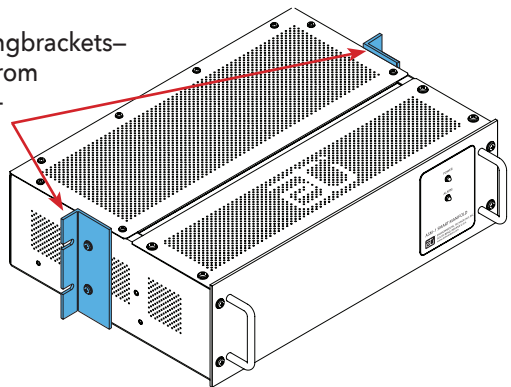
FIGURE 10. Mounting Brackets 8-inch Depth Position
