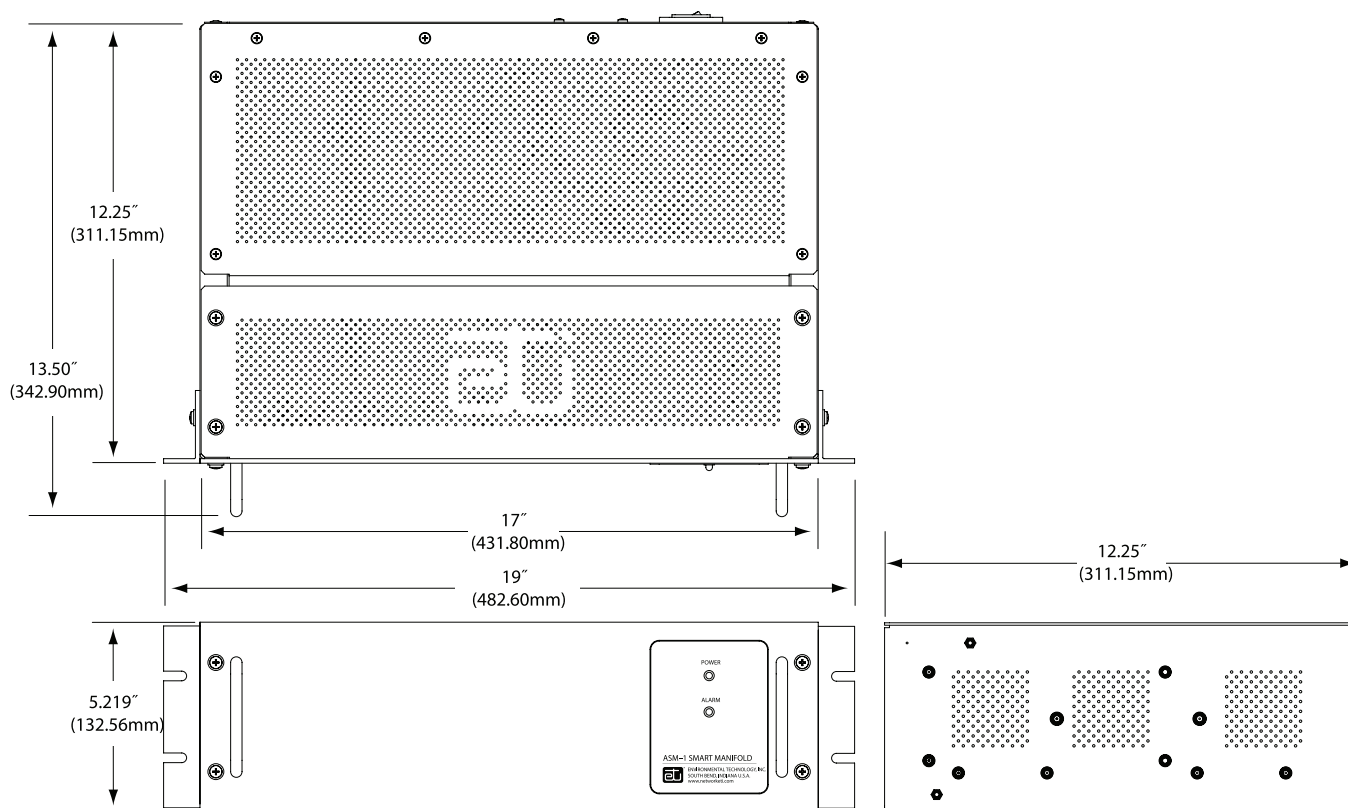
FIGURE 4. ASM-1 Smart Manifold Rack Mounting Dimensions.
