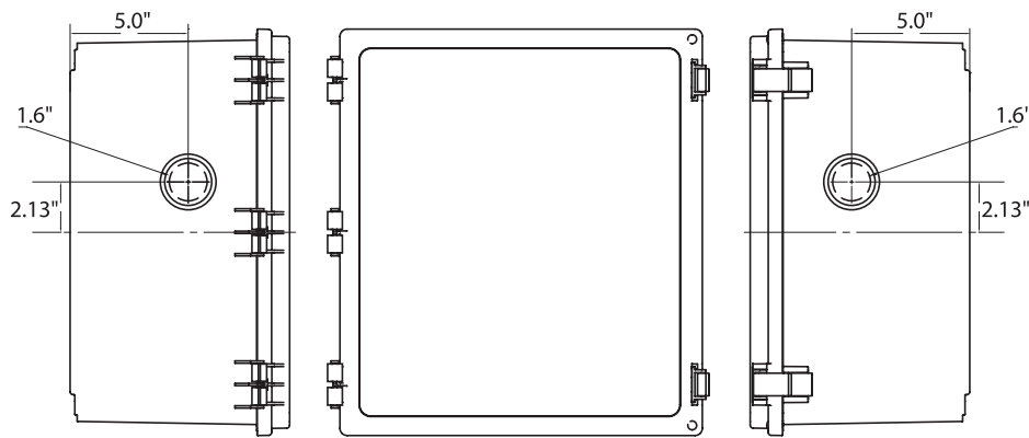
FIGURE A2. Smart Manifold AC NEMA Enclosure Dimensions. (Standard AC NEMA enclosure configuration shown above)
