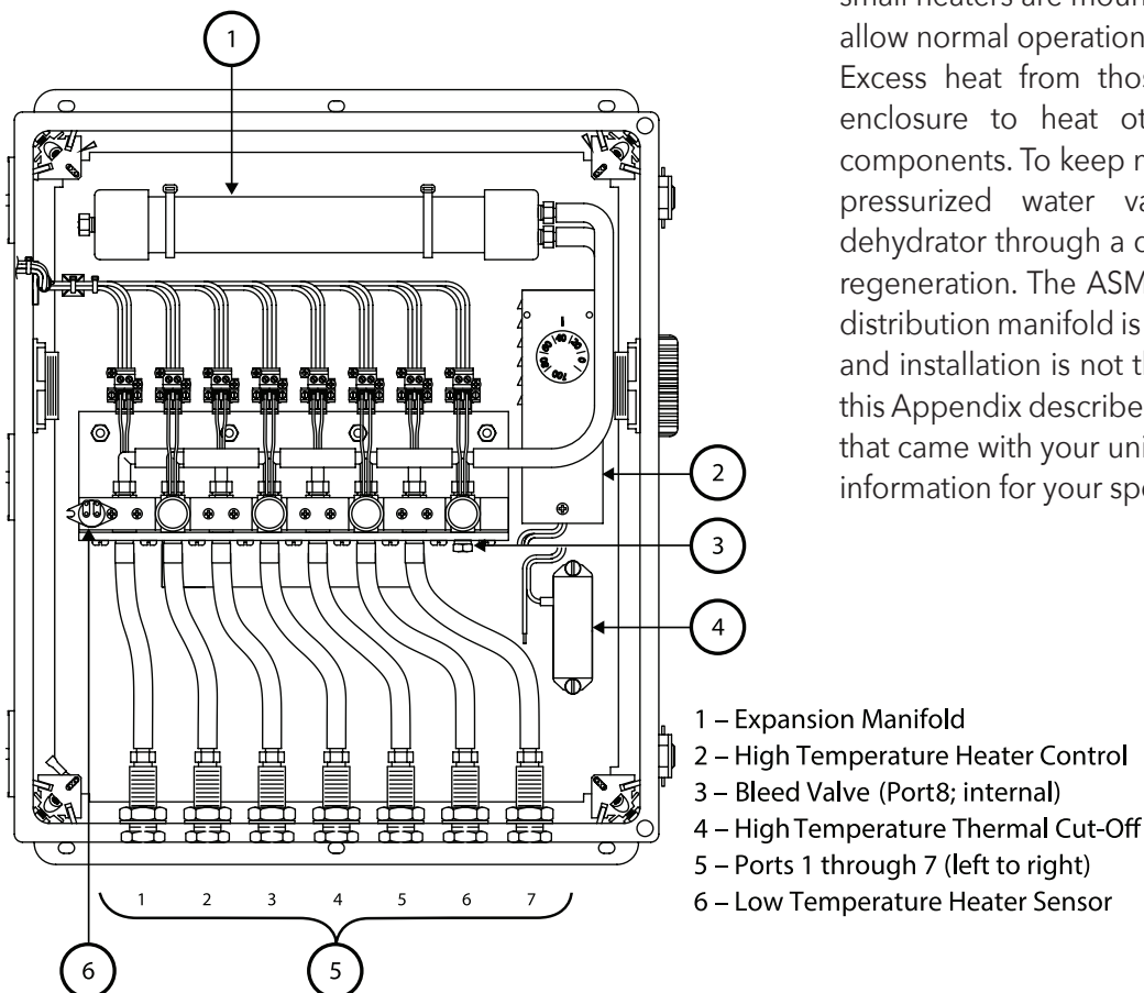
FIGURE A1. ASM-1 Smart Manifold AC NEMA components.
