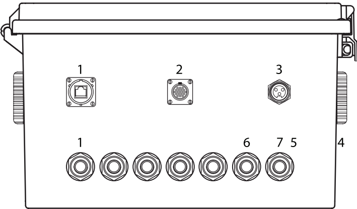
FIGURE A4. Smart Manifold AC NEMA Communication Ports.
