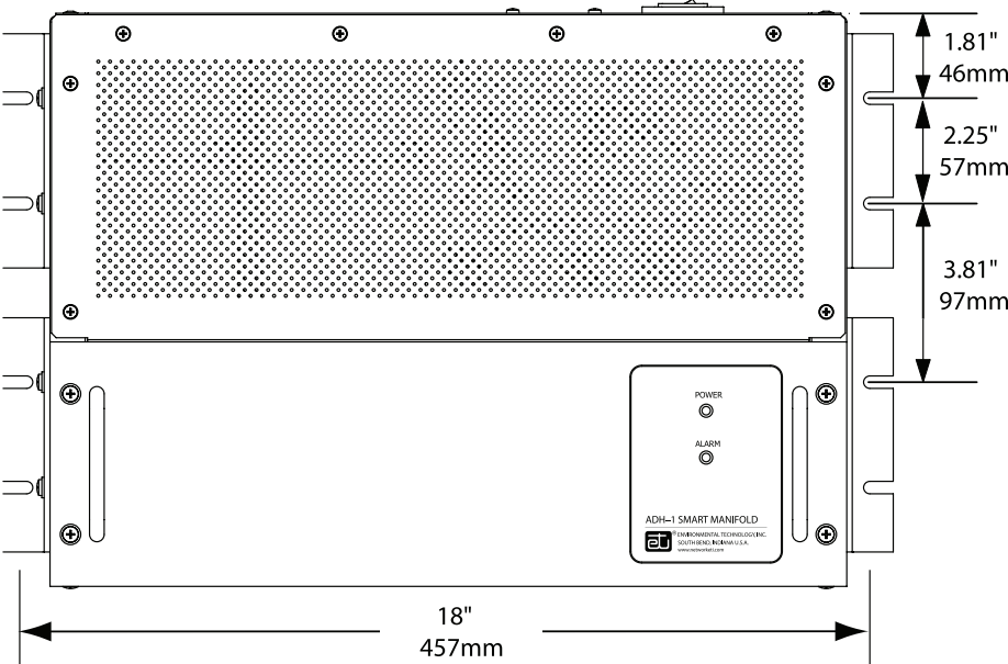
FIGURE 14. ASM-1 Smart Manifold Wall Mount Point Dimensions.
