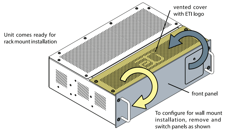
FIGURE 11. ASM-1 Wall Mount Conversion.
