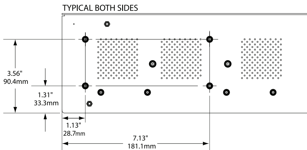
FIGURE 5. ASM-1 Smart Manifold Rack Mount Hole Dimensions.
