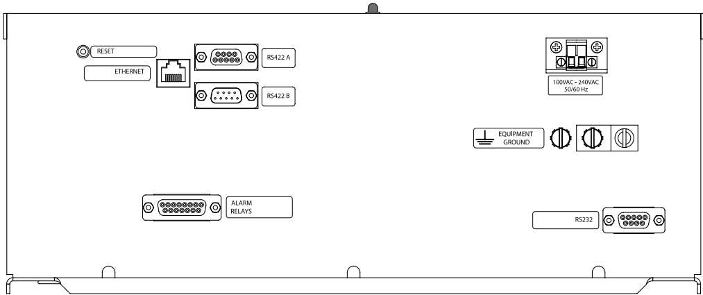
FIGURE A5. Cable Connection Locations.
