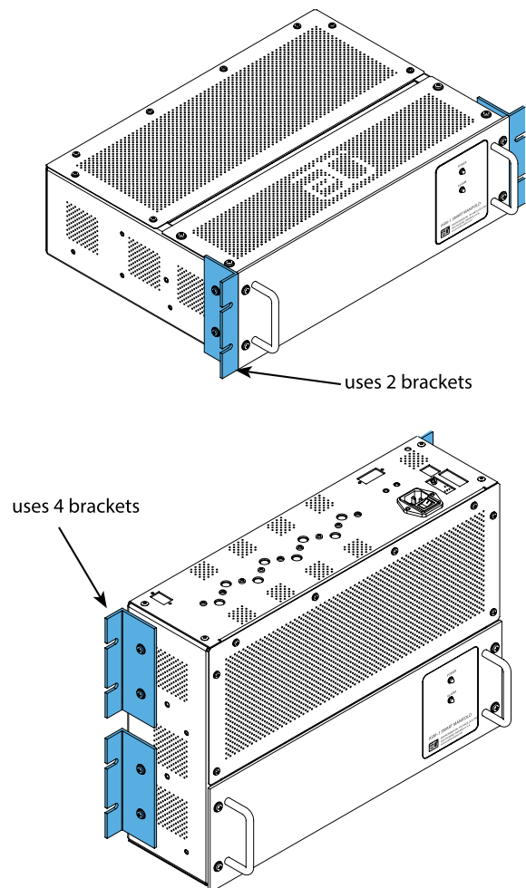
FIGURE 3. ASM-1 Rack Mount (top) and Wall Mount (bottom) configurations.
