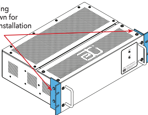
FIGURE 9. Mounting Brackets 6-inch Depth Position
